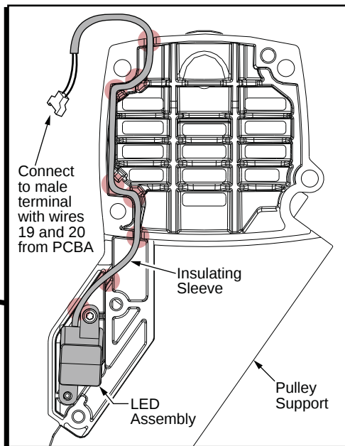
BACK VIEW (INSIDE) OF PULLEY SUPPORT
