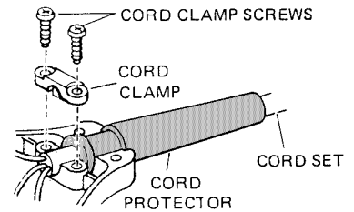
CORD CLAMP DETAILS
