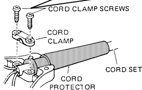
CORD CLAMP DETAILS
